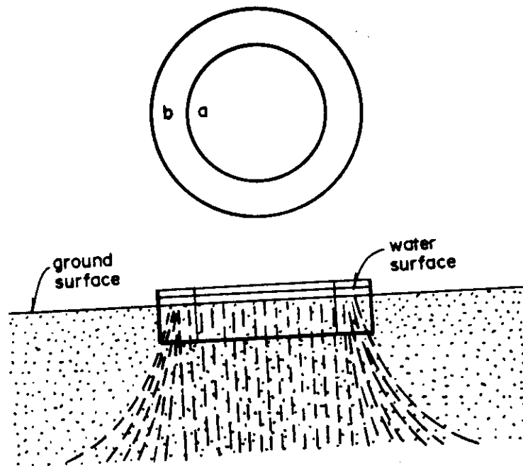
Figure D-3 TWO-RING INFILTROMETER
