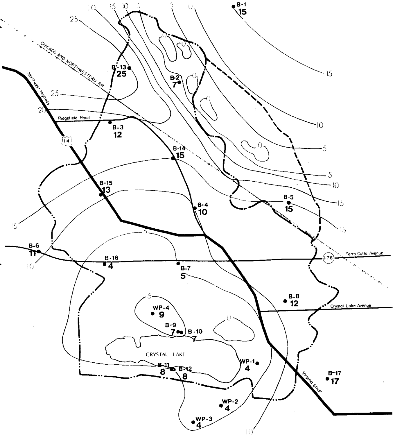
Figure II-3A WELL LOCATIONS
