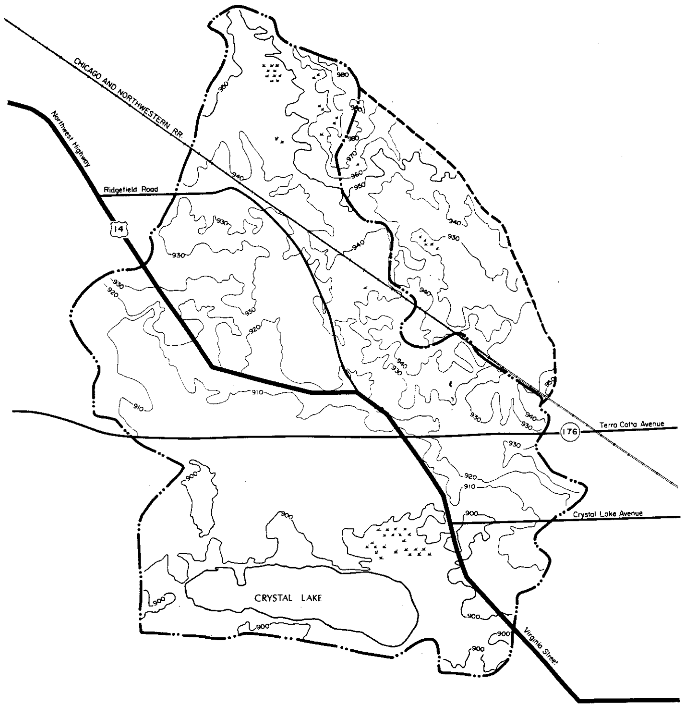
Figure II-4 TOPOGRAPHY
