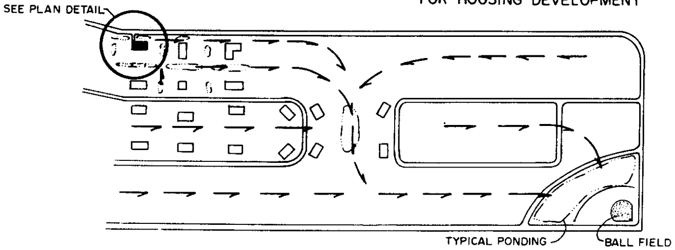
30-ACRE DEVELOPED AREA SHOWING INDIVIDUAL LOT AND GENERAL AREA DRAINAGE FLOW
