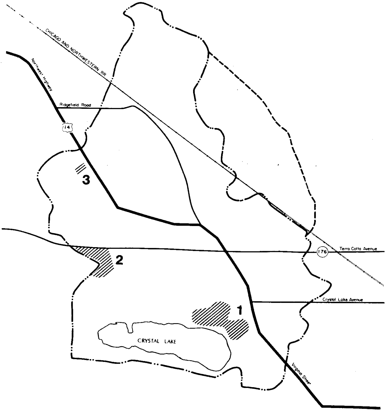
Figure II-8 NATURAL AREAS
