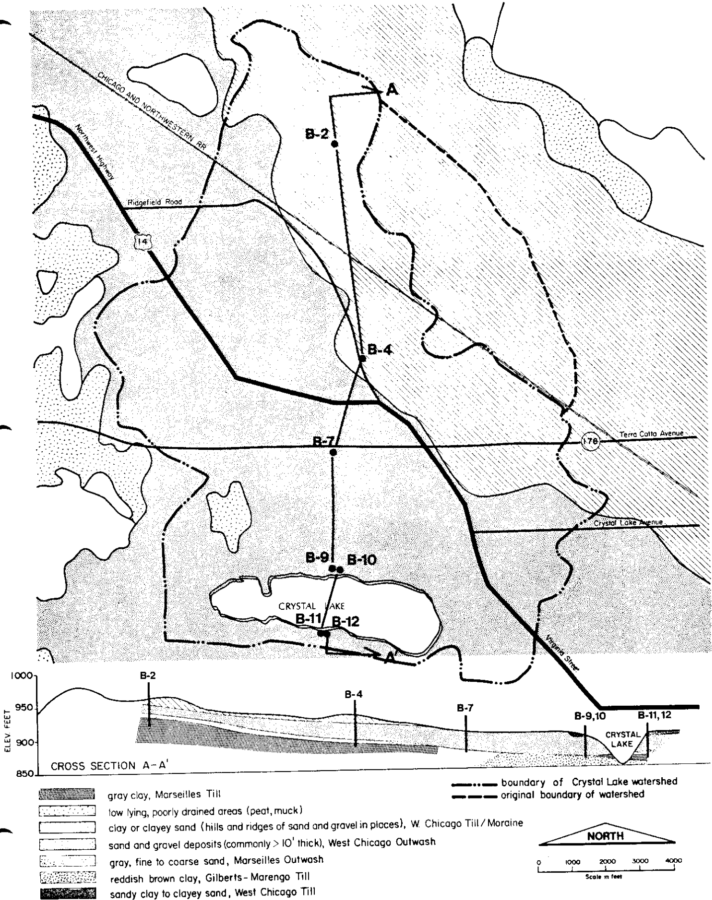
Figure II-3 SURFICIAL GEOLOGY
